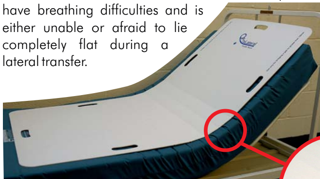
QProLateral Size 1500mm Long x 740mm Wide x 4.5 mm Thick
